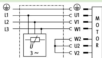
Varistor-suppression (estrela)
